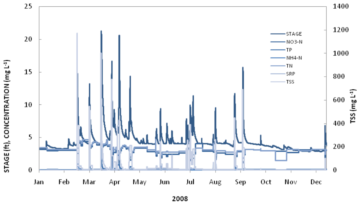
Figure 1. Continuous discharge with constituent concentrations extended to midpoint to determine annual loads for 2008 at the Illinois River at AR Highway 59 Bridge, northwest Arkansas.
